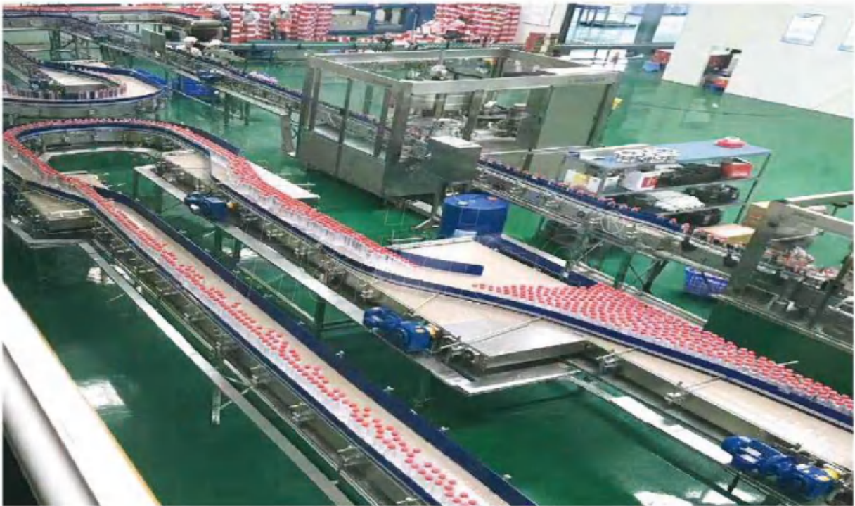
Production Line
